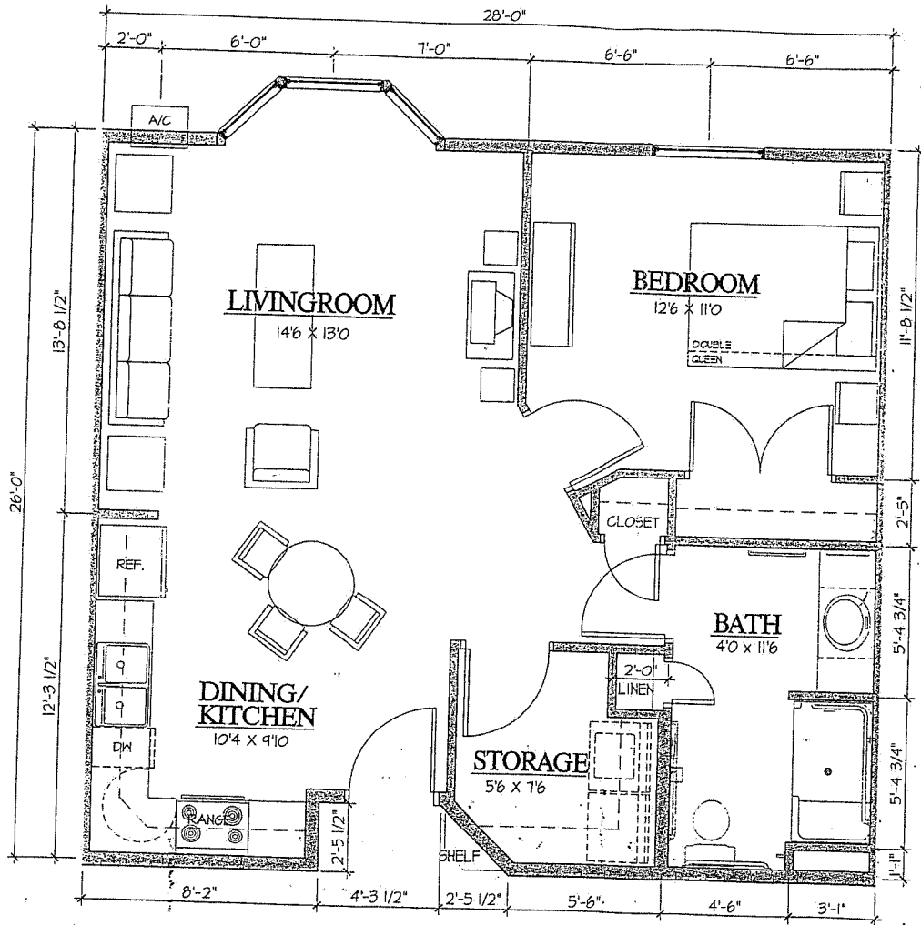
1 ONE BEDROOM UNIT (733 SQ. FT.) "A" SCALE: 1/4"=1'-0"
